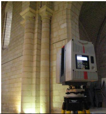
Scanner laser 3D HDS 6000 LEICA
